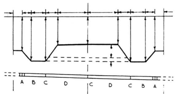
A. Field Drainage Connection. B. 10 Ft. Perforated Corrugated Metal Pipe Unless Otherwise Approved. C. Connection Using Standard Approved Bands, Or Other Devices. D. 20 Ft. Solid Corrugated Metal Pipe Unless Otherwise Approved.
